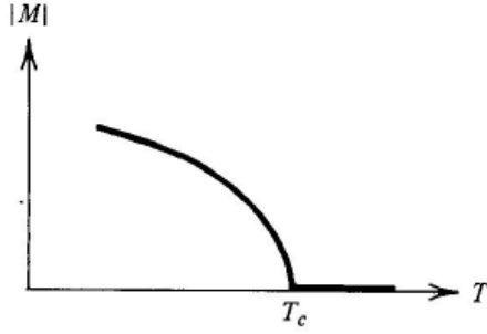
Fig. 5.2. Spontaneous magnetization.
